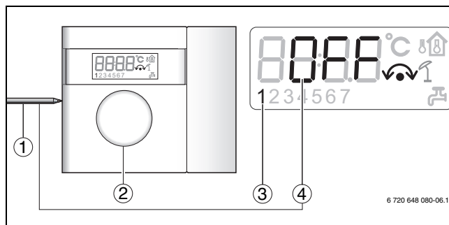
Fig. 23 Terminer le bus CAN LCD
