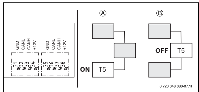
Fig. 16 Terminering CANbus LCD
